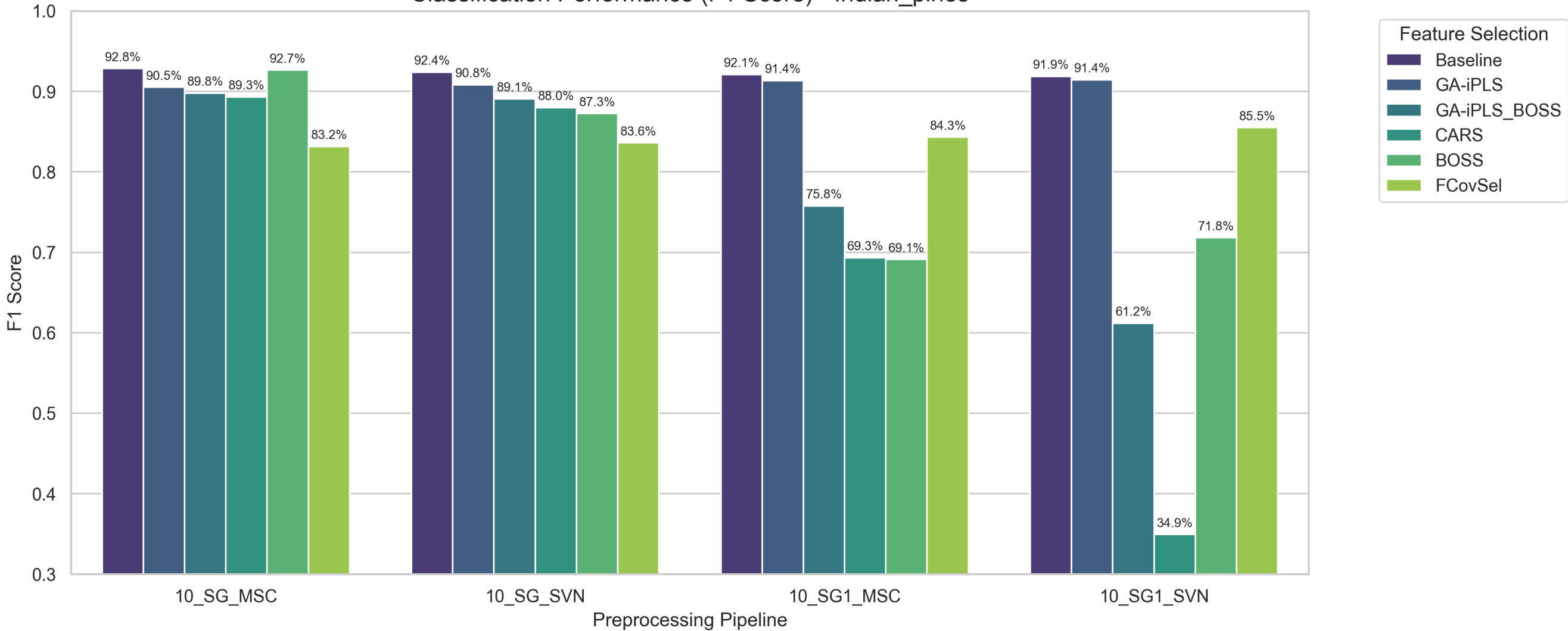
Classification Performance (F1 Score) - Indian_pines
